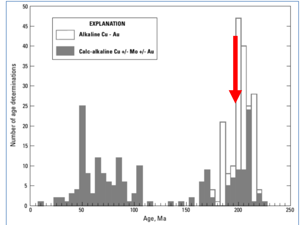
Histogram showing frequency distribution of ages of Canadian porphyry copper deposits
